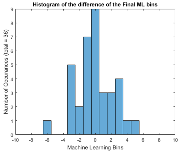
Fig. 7. Histogram of consistency of ML
