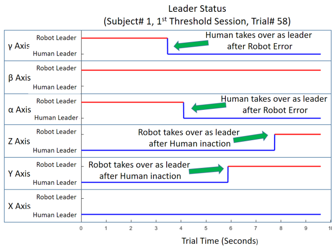
Fig. 5. Leader Status - Human starts as leader of translational DOF and as follower of rotational DOF
