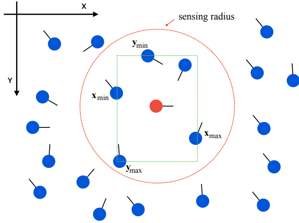
Fig. 3: The definition of the surround rectangle R used in the surround behavior is shown. The sensing radius concentric to the red agent, highlighted red only for visualization purposes, encapsulates five neighboring agents. R is constructed from the local minimum and maximum coordinates as shown by the x_{min} , y_{min} , x_{max} , and y_{max} labels.
