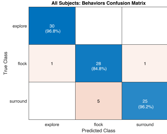
Fig. 8: Combined confusion matrix of all six subjects using the three behaviors as separate classes. The model was trained and tested for each subject with the classification results added together. Out of 90 total observations, the explore , flock , and surround behaviors were correctly predicted 96.8%, 84.8%, and 96.2% of the time, respectively.
