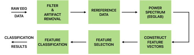
Fig. 4: EEG processing workflow.
