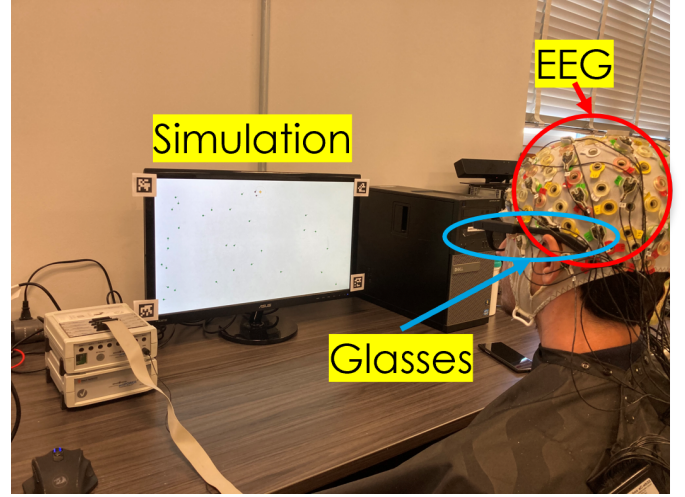
Fig. 1: Experimental setup. A subject is wearing an EEG cap and gaze-tracking glasses while viewing the computer screen during a swarm simulation.
