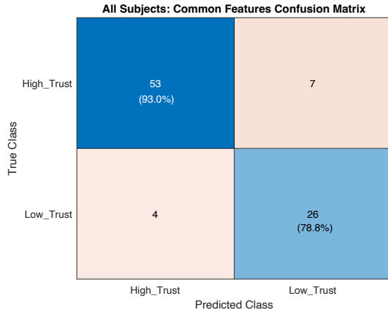
Fig. 10: Combined confusion matrix of all six subjects using the trust classes. The model was trained with the six most common features, see Table III, found in at most four subjects. The classification results are added together. Out of 90 total observations, the low-trust and high-trust conditions were correctly predicted 78.8% and 93.0% of the time, respectively.
