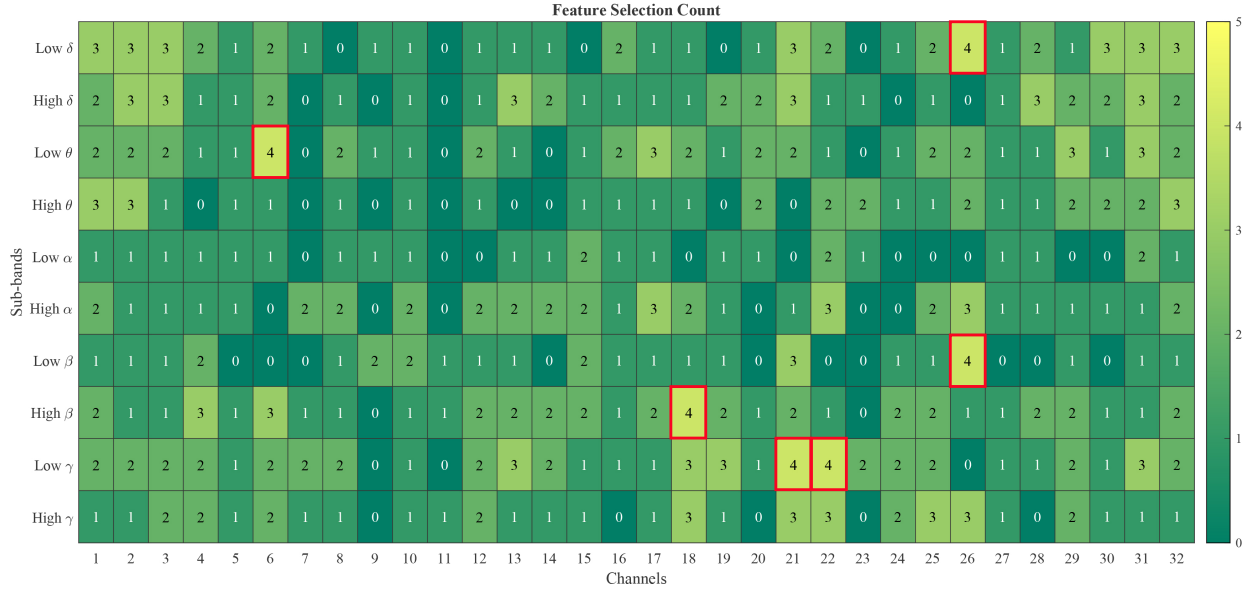
Fig. 9: Commonality of selected features across all six subjects represented as a heatmap. The features are described by sub-band (rows) and channel (columns). Each feature or cell a subject has will be counted as one. The maximum value a cell can have is six. The common features among 4 subjects are highlighted by a red box around them.
