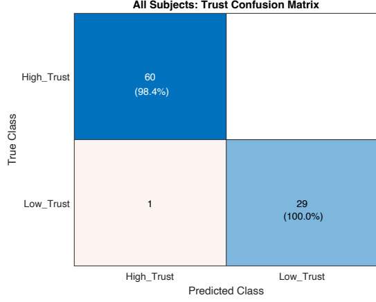
Fig. 7: Combined confusion matrix of all six subjects using the low- and high-trust classes. The model was trained and tested for each subject with the classification results added together. Out of 90 total observations, the low-trust and high-trust conditions were correctly predicted 100.0% and 98.4% of the time, respectively.
